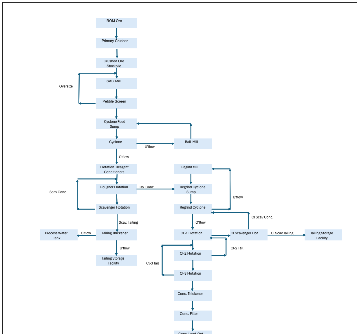
Figure 4. Processing Circuit
